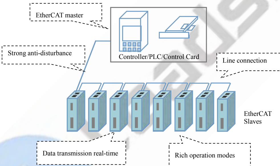
Figure 1.2: EtherCAT Topology
