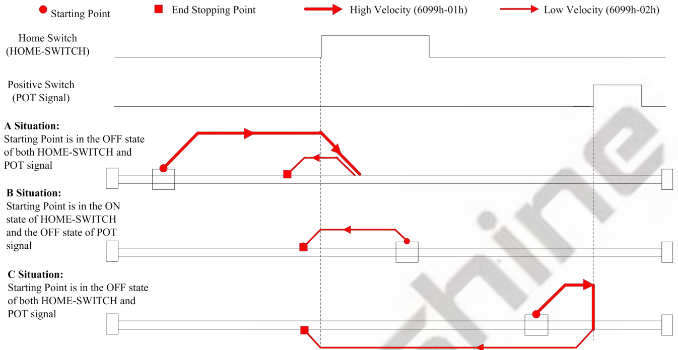
Figure 8.7 No.23 homing method
