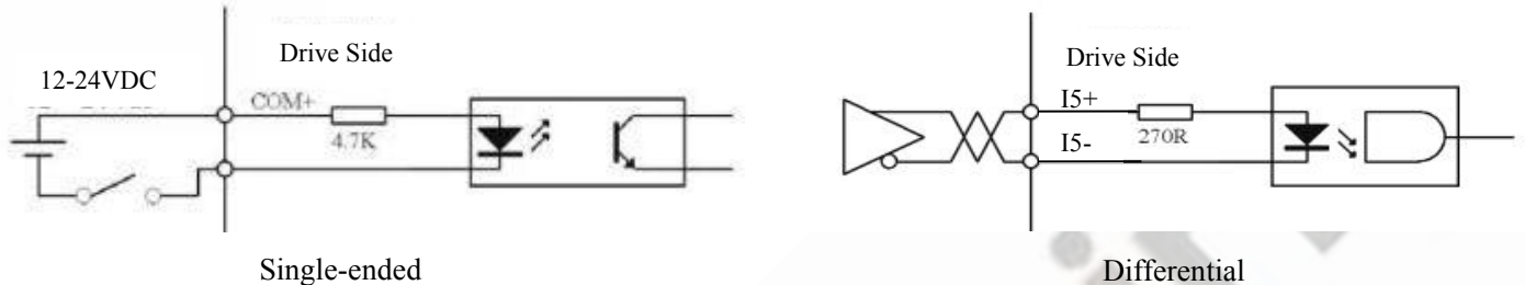
Figure 3.3 Input Interface Wiring
