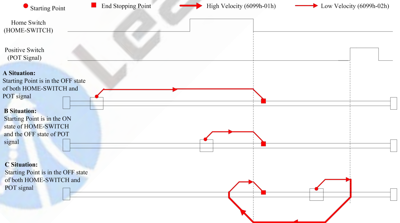
Figure 8.10 No.26 homing method
