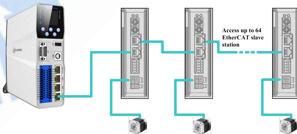
Figure 6.1 EM3E series network diagram
