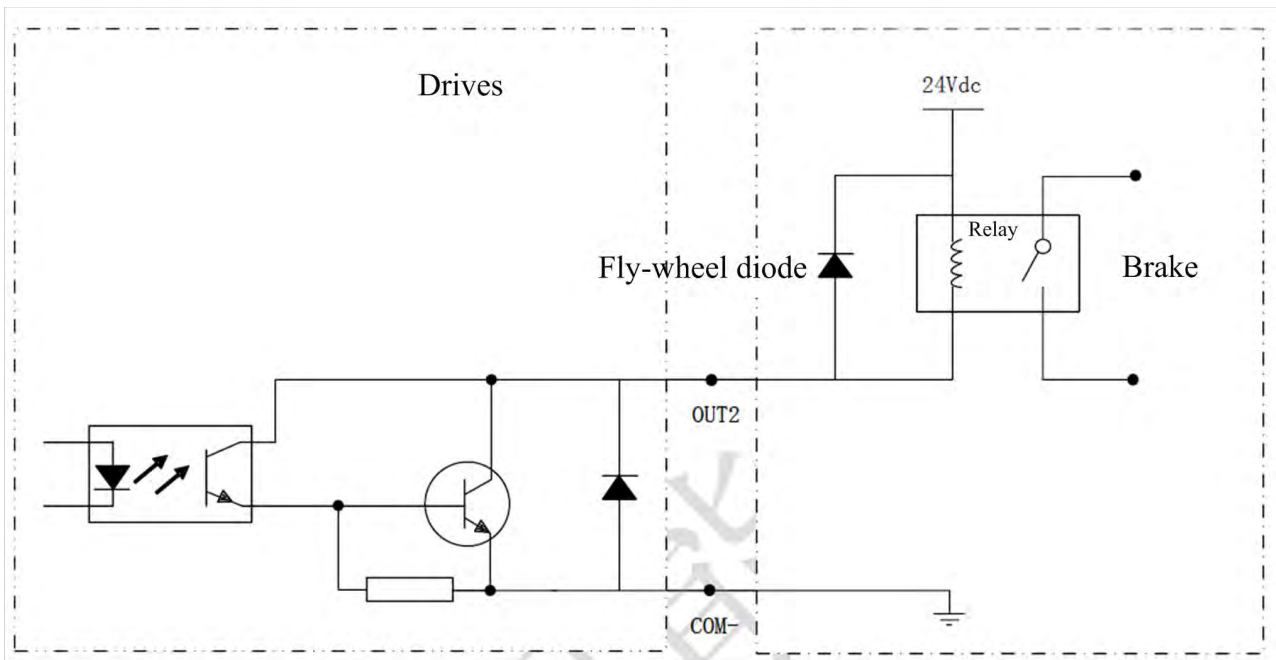
Figure 3.5 Brake Output Wiring
