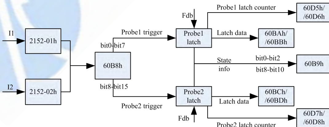
Figure 5.8 Touch probe function
