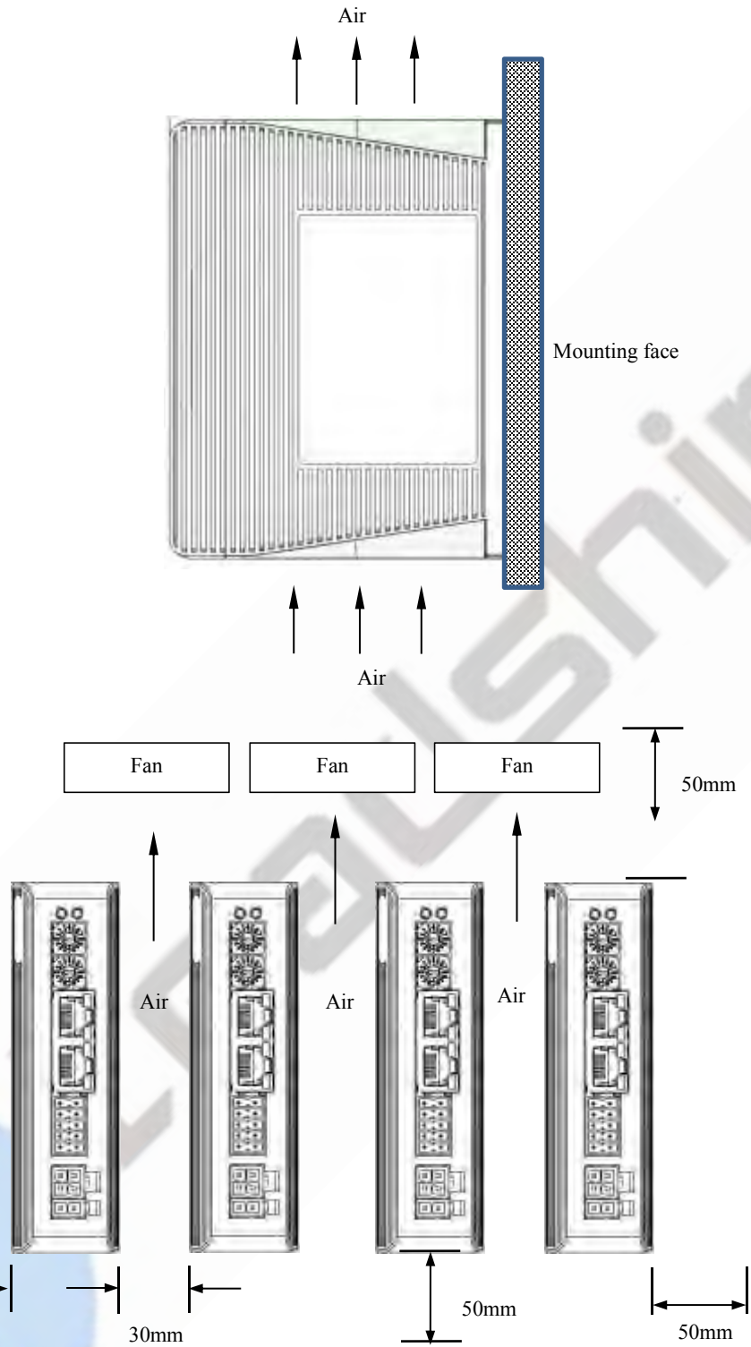
Figure 2.2 EM3E series installation drawing
