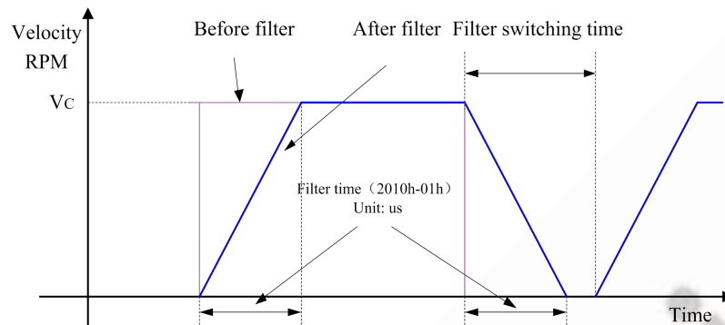
Figure 5.4 Filtering effect for square wave command
