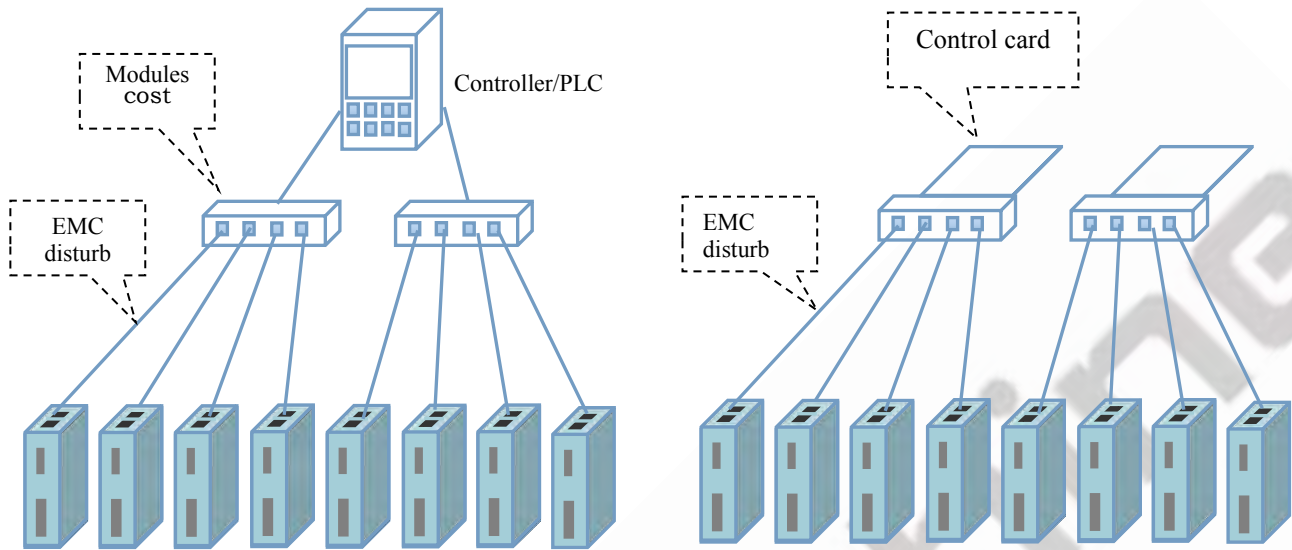
Figure 1.1: Step/direction Topology
