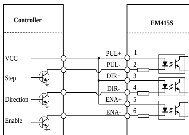
Figure 4 Connections to PNP signals (Common-cathode)
